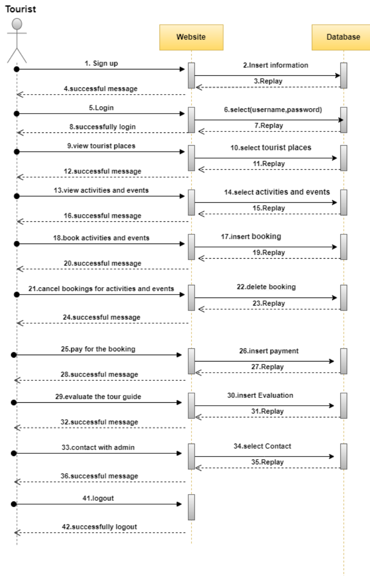
Figure 3. 5: Sequence Diagram for Tourist
