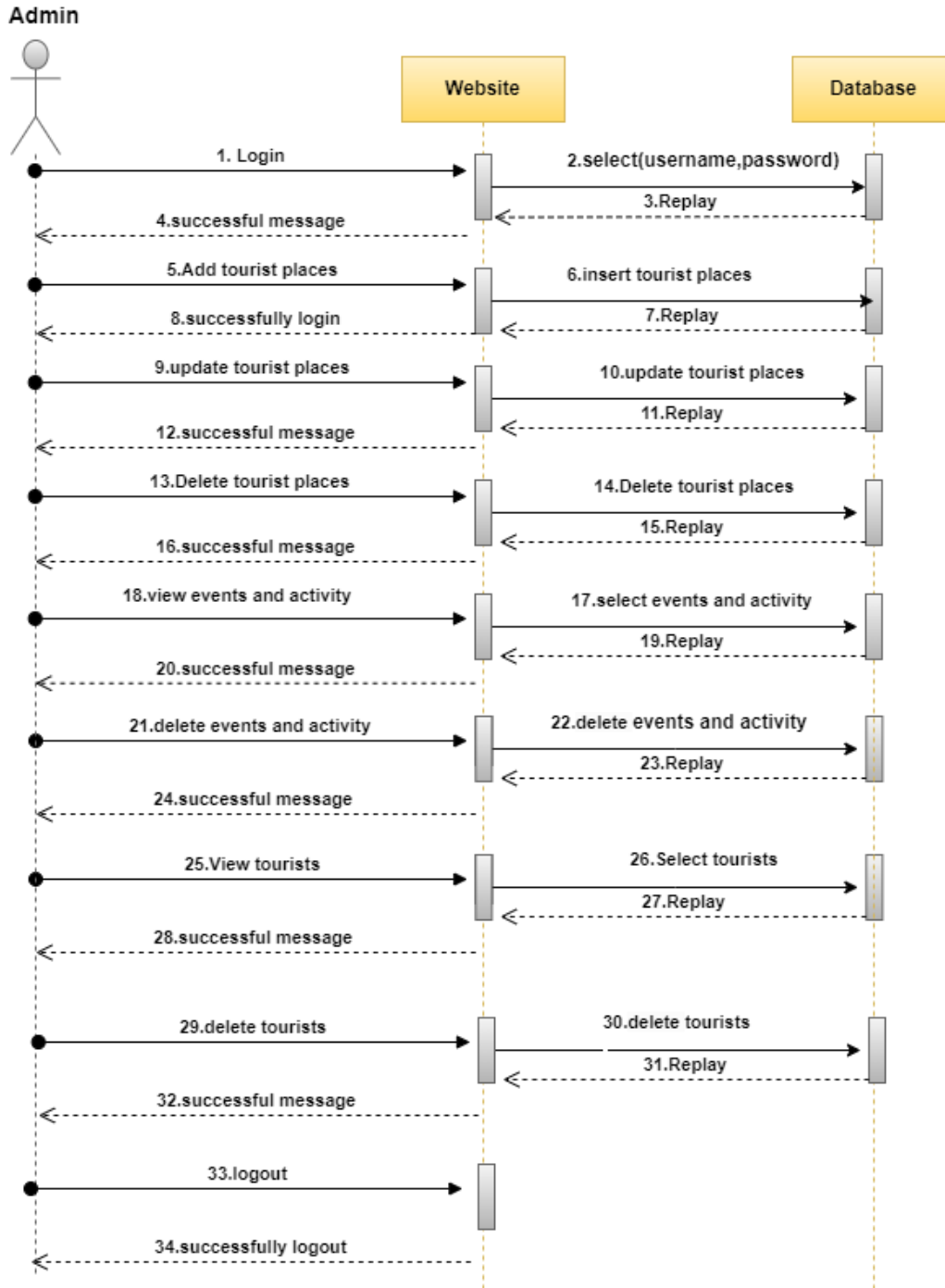
Figure 3. 7: Sequence Diagram for Admin
