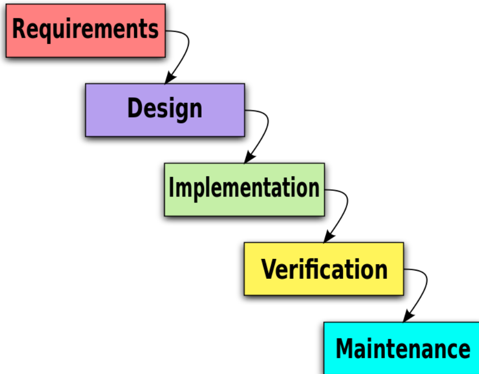
Figure 1. 1: METHODOLOGY
