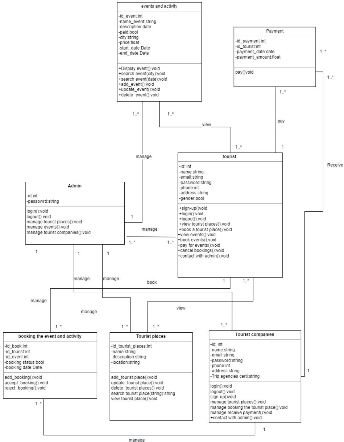
Figure 3. 8: CLASS DIAGRAM
