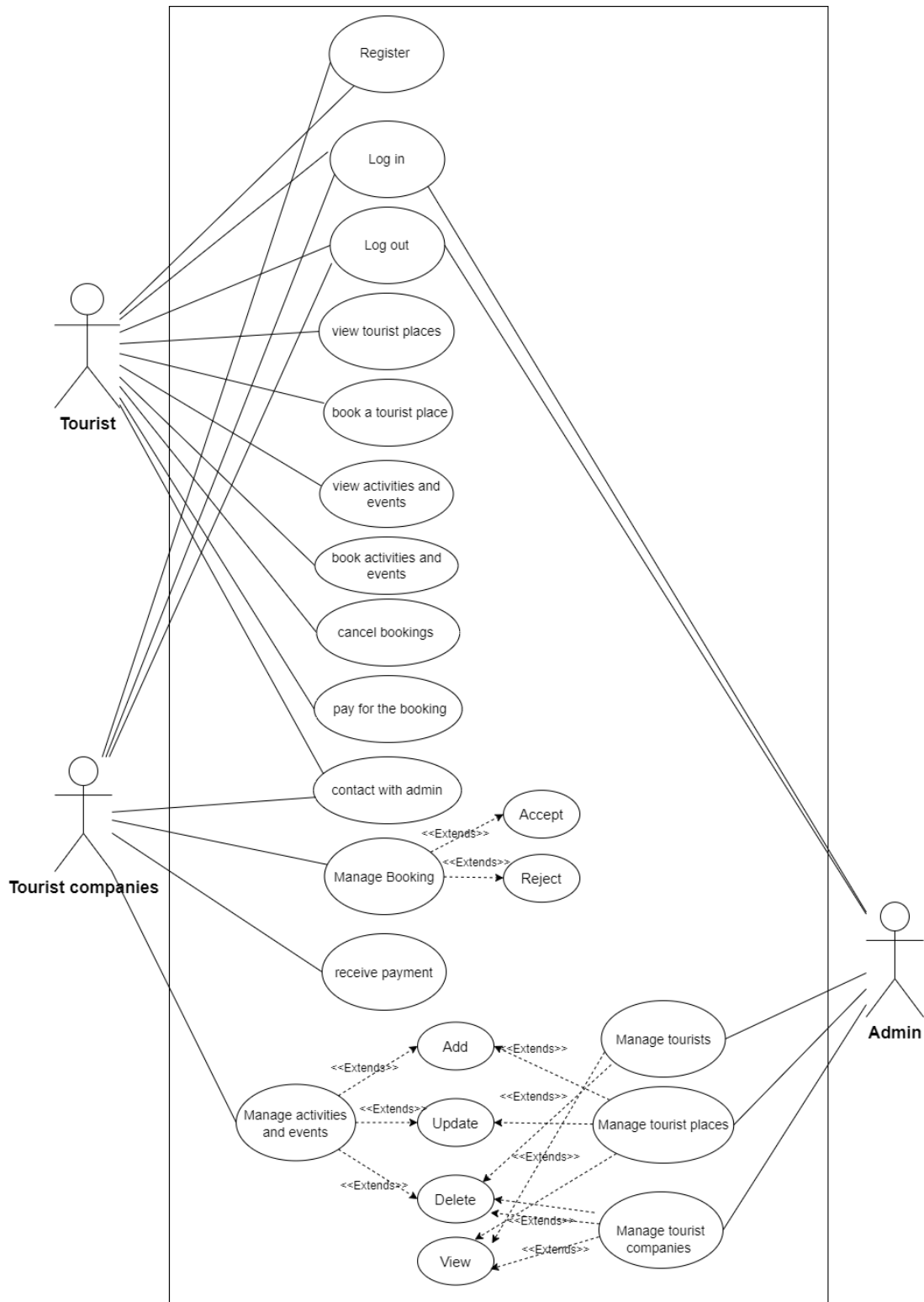
Figure 3. 4: Use Case Diagram for System
