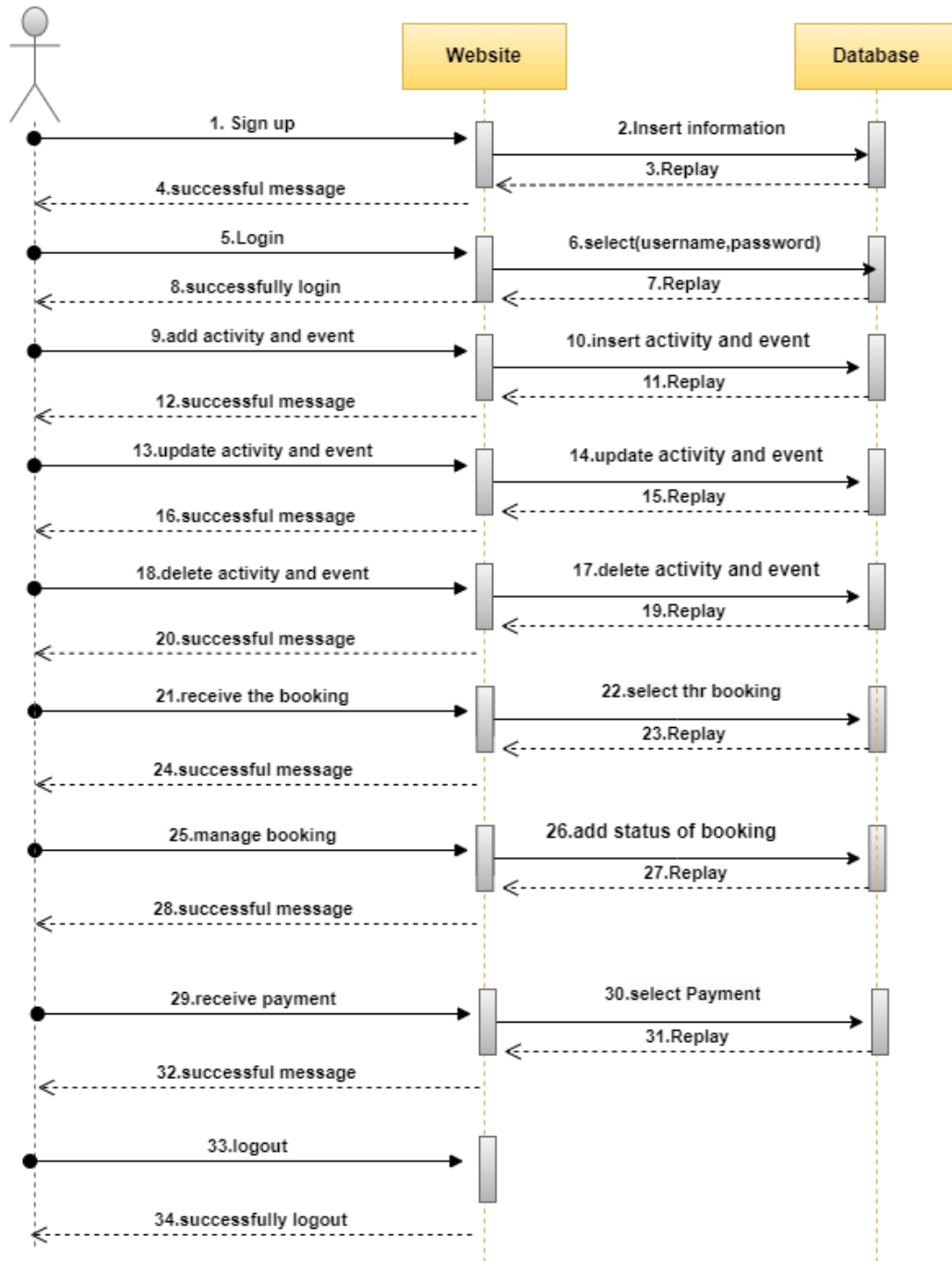
Figure 3. 6: Sequence Diagram for Tourist Companies
